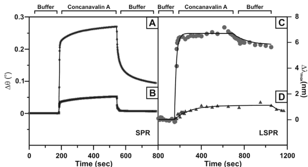
Figure 4. Real-time response of sugar-functionalized sensor as 19 \mu\text{M} of ConA was injected in the cell following buffer injection. (A) mannose-functionalized SPR sensor, (B) galactose-functionalized SPR sensor, (C) mannose-functionalized Ag nanosensor, and (D) galactose-functionalized Ag nanosensor. The points are the experimental data. The solid line for the SPR measurement is composed of straight line segments connecting the experimental data. The solid line in LSPR measurement is a first-order adsorption kinetics fit to the data and should only be interpreted as a guide to the eye.
