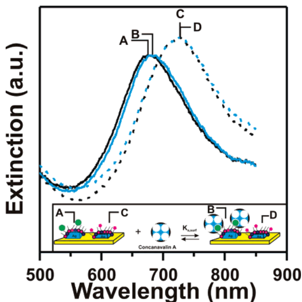
Figure 9. LSPR spectra illustrating multiplexing Ag nanosensor carbochip. Ag nanobiosensor with 35 nm Ag and 75 nm Ag were fabricated using NSL. (A) Ag nanoparticles (height = 75 nm) after 5 mM mannose modification, \lambda_{\max} = 677.7 nm. (B) Ag nanoparticles (height = 75 nm) after exposure to 19 \mu\text{M} ConA, \lambda_{\max} = 682.7 nm. (C) Ag nanoparticles (height = 35 nm) after 5 mM galactose modification, \lambda_{\max} = 724.5 nm. (D) Ag nanoparticles (height = 35 nm) after exposure to 19 \mu\text{M} ConA, \lambda_{\max} = 724.6 nm. Inset shows the schematic of selective ConA binding to the mannose-functionalized portion of the carbochip.
