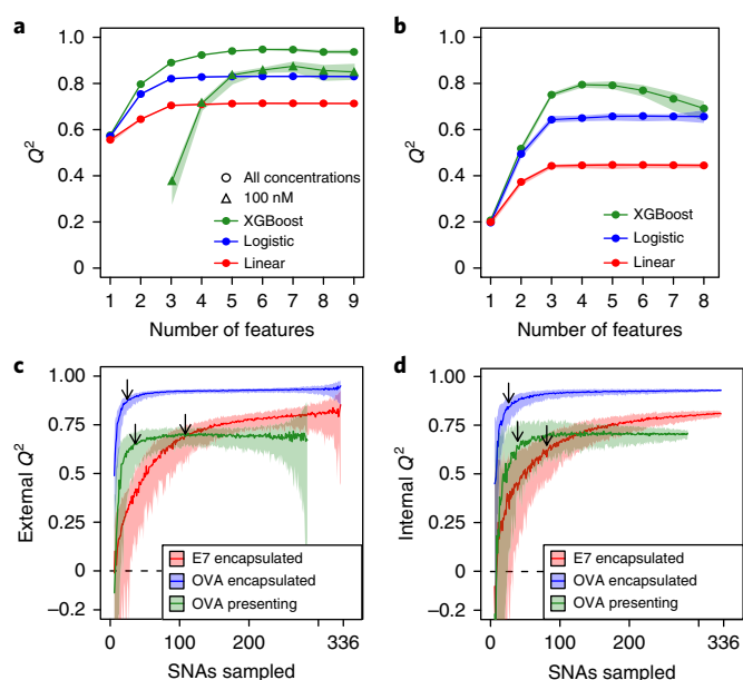
Fig. 6 | Analysis by machine learning. a, b , Q^2 values of the highest-performing SNA property combinations are shown across different numbers of properties for encapsulated OVA ( a ) and surface-presented OVA subsets ( b ). In a , for the XGBoost model, the active sequence and 100 nM subset is shown, in addition to both active and inactive sequences for all concentrations. c, d , XGBoost Q^2 performance when selecting and training on a random SNA subsample and testing predictions on the unselected SNAs ( c ) or cross-validating within the selected subsample ( d ). The shading represents 90% confidence intervals. The arrows point to the points of diminishing returns.
