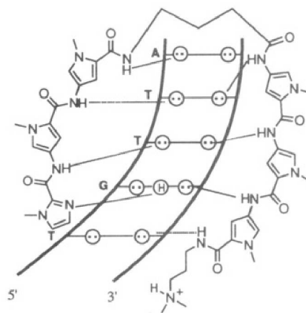
Figure 8. Model for the complex formed between the hexapeptide 2-ImN-GABA-P3 and the 5'-TGTTA-3' site. Circles with dots represent lone pairs of N3 of purines and O2 of pyrimidines. Circles containing an H represent the N2 hydrogen of guanine. Putative hydrogen bonds are illustrated by dotted lines.
