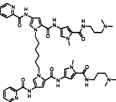
1d: (2-PyN) 2 -C6
