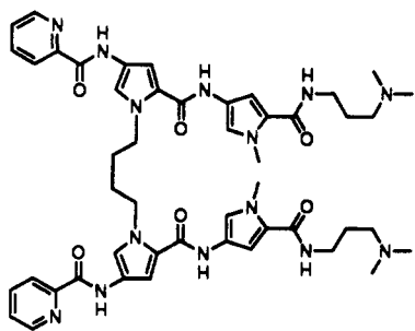
1b: (2-PyN) 2 -C4
