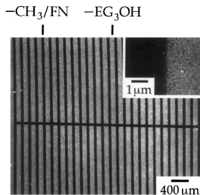
FIG. 4. Fibronectin (100 \mu\text{g/mL} in PBS) was allowed to adsorb to a patterned SAM for 2 h. The pattern of protein was characterized by scanning electron microscopy. The layer of protein attenuates secondary electron emission and appears as the dark areas in the micrograph. The inset shows a view at higher magnification and demonstrates the edge resolution of the pattern of protein.
