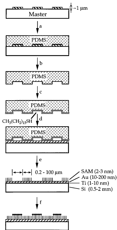
FIG. 2. Microcontact printing ( \mu CP) can pattern the formation of SAMs with dimensions down to 1 \mu\text{m} . A poly(dimethylsiloxane) (PDMS) stamp is fabricated by casting the prepolymer against a master pattern (a) to give a stamp having a complementary pattern of relief (b). The stamp is "inked" with an alkanethiol (c) and brought into conformal contact with a surface of gold (d). A SAM of alkanethiolates is formed only at those regions where the stamp contacts the surface (e); the bare regions of gold remaining after the printing process can be modified with a different SAM by immersing the substrate in a solution of a second alkanethiol (f).
