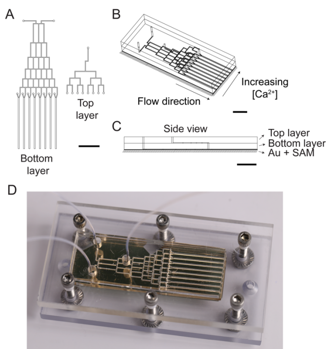
Figure 2. Microfluidic device layers and assembly with A) bottom view of both layers, B) the assembled device, and C) side view. D) Device and clamp assembly. All scale bars = 5 mm.
