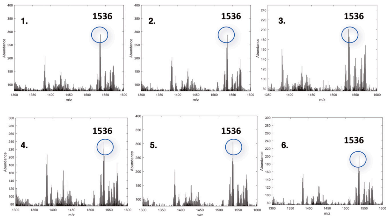
Fig. 3. (A) Scaled-up hit reactions (0.1 mmol E1 , 0.15 mmol Bn HEH ). (B) Hit spectra for entries 1–6.
